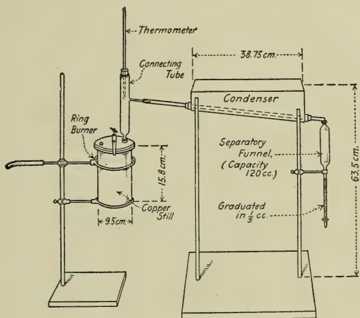
FIG. 188.—Still for Determining Water.
